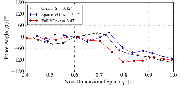
Figure 17: Phase variation at 216 Hz for the three configurations above buffet onset.
