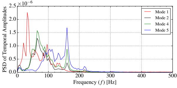
(a) Clean configuration at buffet onset, \alpha = 2.73^\circ .
