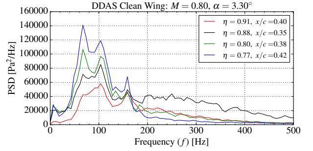
Figure 4: PSDs corresponding to the shock along the span, \alpha = 3.30^\circ
