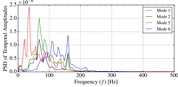
(b) Sparse VG configuration at buffet onset, \alpha = 2.91^\circ .
